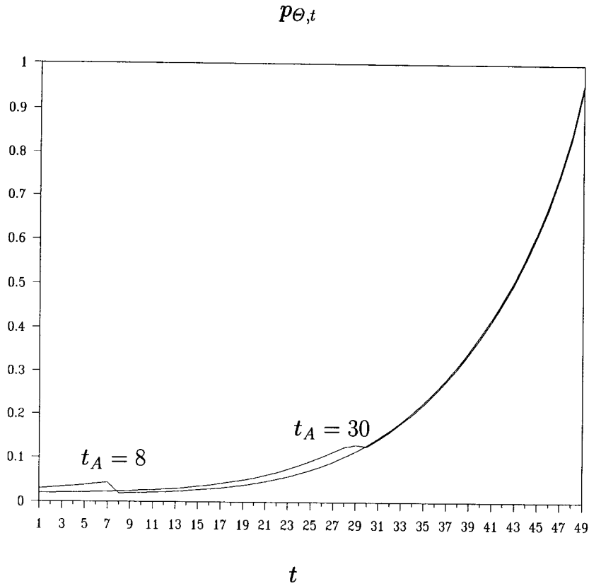
Figure 7 Coefficient of the price function p_{\Theta,t} when there is a public announcement This figure plots the time path of p_{\Theta,t} , the coefficient of total stock supply \Theta_t in the price function, when there is a public announcement. The parameters are set at the following values: T = 50 , \lambda = 2.0 , a_{\Theta} = 0.85 , \sigma_{\Pi}^2 = 0.35 , \sigma_{\Theta}^2 = 0.1 , \sigma_{\delta}^2 = 0.25 , \sigma_{S,1}^2 = 2.0 , \sigma_{S,t}^2 = 10^6 ( 1 < t \leq T - 1 ), \sigma_{v,t_A}^2 = 6.0 , \sigma_{v,t}^2 = 10^6 ( t \neq t_A ). The announcement dates are, respectively, t_A = 8 and t_A = 30 .
