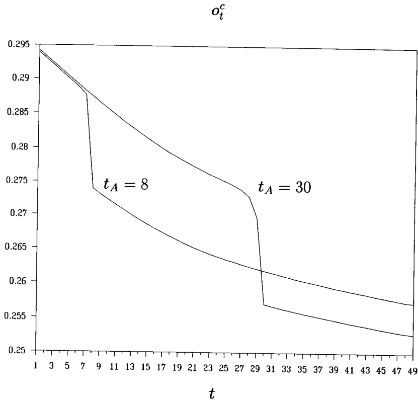
Figure 9 Remaining uncertainty in the underlying value of the stock \Pi when there is a public announcement This figure plots \sigma_t^c , the remaining uncertainty in the underlying value of the stock conditional on investors' information, over time when there is a public announcement. The parameters are set at the following values: T = 50 , \lambda = 2.0 , \alpha_\omega = 0.85 , \sigma_\Pi^2 = 0.35 , \sigma_\theta^2 = 0.1 , \sigma_\delta^2 = 0.25 , \sigma_{s,1}^2 = 2.0 , \sigma_{s,t}^2 = 10^6 ( 1 < t \leq T - 1 ), \sigma_{y,t_A}^2 = 6.0 , \sigma_{y,t}^2 = 10^6 ( t \neq t_A ). The announcement dates are, respectively, t_A = 8 and t_A = 30 .
