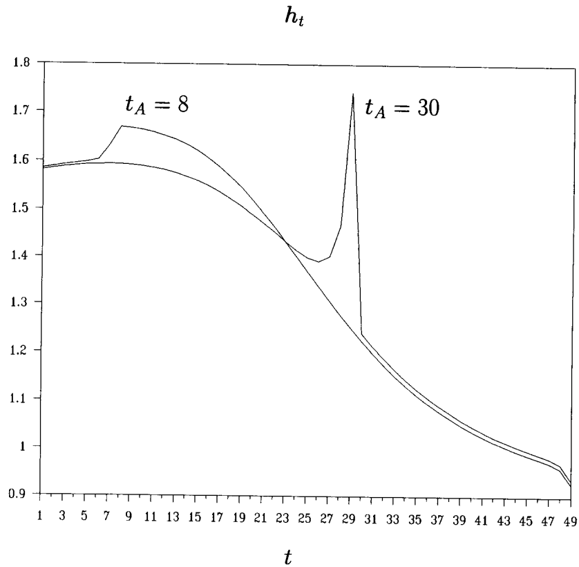
Figure 5 Intensity of investors speculative trading when there is a public announcement This figure plots the intensity of investors speculative trading h_t over time when there is a public announcement. The parameters are set at the following values: T = 50 , \lambda = 2.0 , a_\Theta = 0.85 , \sigma_\Pi^2 = 0.35 , \sigma_\Theta^2 = 0.1 , \sigma_\delta^2 = 0.25 , \sigma_{s,1}^2 = 2.0 , \sigma_{v,t}^2 = 10^6 ( 1 < t \leq T - 1 ), \sigma_{v,t_A}^2 = 6.0 , \sigma_{v,t}^2 = 10^6 ( t \neq t_A ). The announcement dates are, respectively, t_A = 8 and t_A = 30 .
