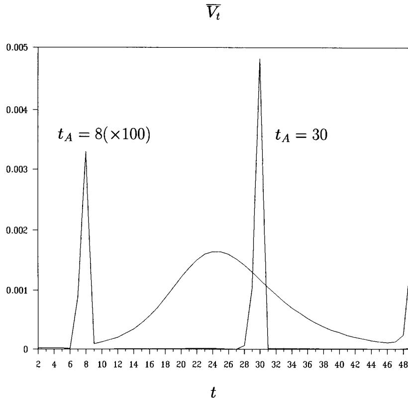
Figure 4 Expected volume of informational trading when there is a public announcement This figure plots the expected volume of informational trading \bar{V}_t over time when there is a public announcement. The parameters are set at the following values: T = 50 , \lambda = 2.0 , a_\theta = 0.85 , \sigma_\Pi^2 = 0.35 , \sigma_\theta^2 = 0.1 , \sigma_\delta^2 = 0.25 , \sigma_{\delta,1}^2 = 2.0 , \sigma_{\delta,t}^2 = 10^6 ( 1 < t \leq T - 1 ), \sigma_{V,t_A}^2 = 6.0 , \sigma_{Y,t}^2 = 10^6 ( t \neq t_A ). The announcement dates are, respectively, t_A = 8 and t_A = 30 .
