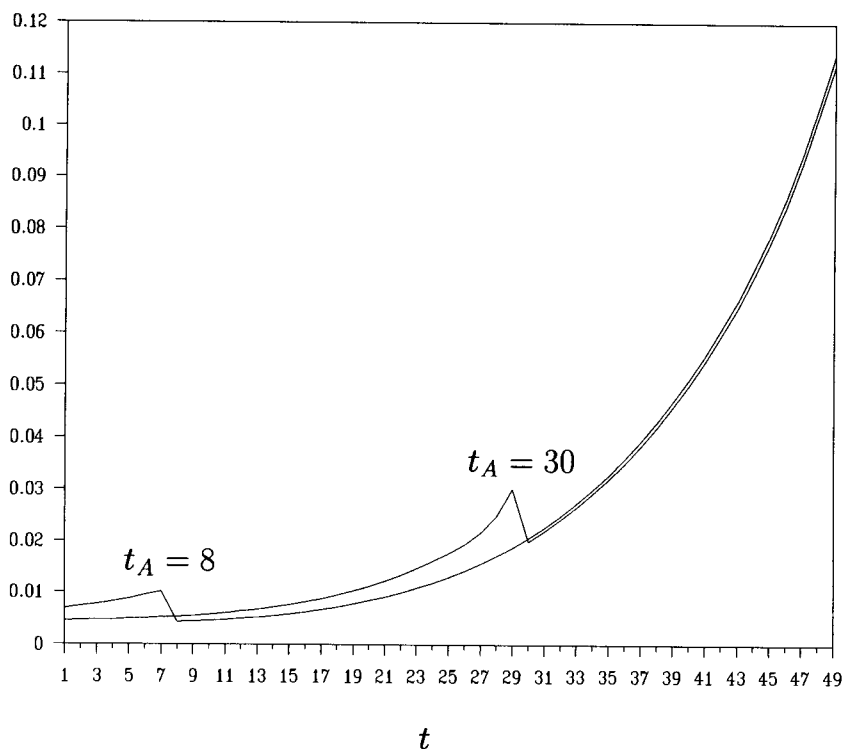
Figure 8 Coefficient of the price function p_{\Pi,t} when there is a public announcement This figure plots the time path of p_{\Pi,t} , the coefficient of underlying stock value \Pi in the price function, when there is a public announcement. The parameters are set at the following values: T = 50 , \lambda = 2.0 , a_{\Theta} = 0.85 , \sigma_{\Pi}^2 = 0.35 , \sigma_{\Theta}^2 = 0.1 , \sigma_{\delta}^2 = 0.25 , \sigma_{S,1}^2 = 2.0 , \sigma_{S,t}^2 = 10^6 ( 1 < t \leq T-1 ), \sigma_{Y,t_A}^2 = 6.0 , \sigma_{Y,t}^2 = 10^6 ( t \neq t_A ). The announcement dates are, respectively, t_A = 8 and t_A = 30 .
