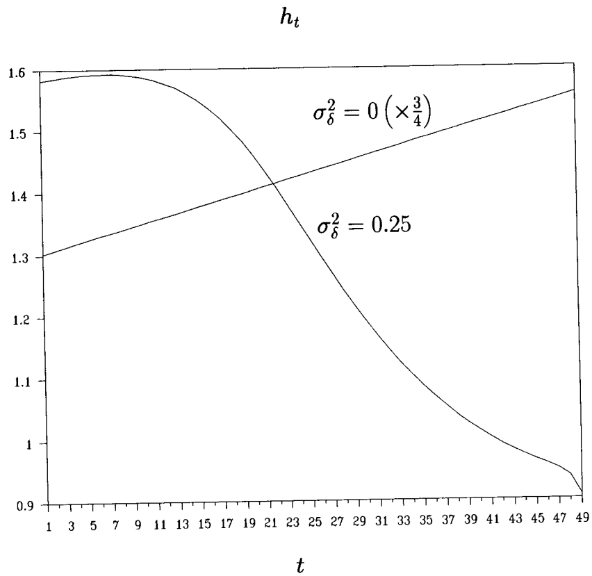
Figure 2 Intensity of investors' speculative trading when there is no public announcement This figure plots the intensity of investors' speculative trading h_t over time in the absence of public announcements. The parameters are set at the following values: T = 50 , \lambda = 2.0 , a_\theta = 0.85 , \sigma_\pi^2 = 0.35 , \sigma_\theta^2 = 0.1 , \sigma_{S,1}^2 = 2.0 , \sigma_{S,t}^2 = 10^6 ( 1 < t \leq T - 1 ), \sigma_{I,t}^2 = 10^6 ( 1 \leq t \leq T - 1 ).
