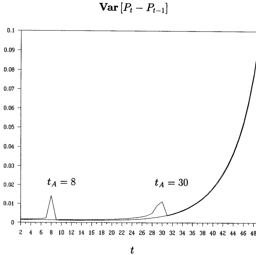
Figure 10 Volatility of price changes when there is a public announcement This figure plots the unconditional volatility of price changes \text{Var}[P_t - P_{t-1}] over time when there is a public announcement. The parameters are set at the following values: T = 50 , \lambda = 2.0 , a_\Theta = 0.85 , \sigma_\Pi^2 = 0.35 , \sigma_\Theta^2 = 0.1 , \sigma_\delta^2 = 0.25 , \sigma_{S,1}^2 = 2.0 , \sigma_{S,t}^2 = 10^6 ( 1 < t \leq T - 1 ), \sigma_{Y,t_A}^2 = 6.0 , \sigma_{Y,t}^2 = 10^6 ( t \neq t_A ). The announcement dates are, respectively, t_A = 8 and t_A = 30 .
