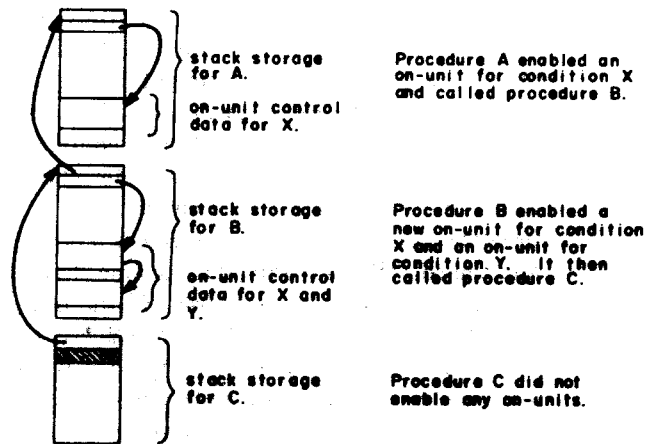
Figure 7—Stack storage and the signal mechanism A signal for condition X causes the signal mechanism to search back through the stack until it finds the first enabled on-unit for condition X. An on-unit is compiled as an internal procedure. The execution of an ON-statement creates a block of on-unit control data. This control data consists of the name of the condition for which the unit was enabled and a procedure variable. The signal mechanism uses the procedure variable to invoke the on-unit. All data associated with the enabled on-unit is stored in the stack storage of the procedure which enabled it. Normal popping of the stack reverts the on-units enabled during the execution of the procedure.
