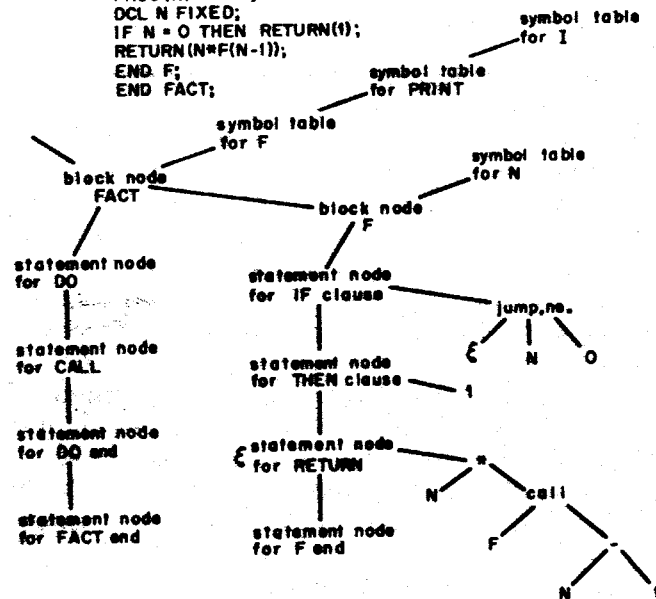
Figure 1—The internal representation of a program. The example is greatly simplified. Only the statements of procedure F are shown in detail.
