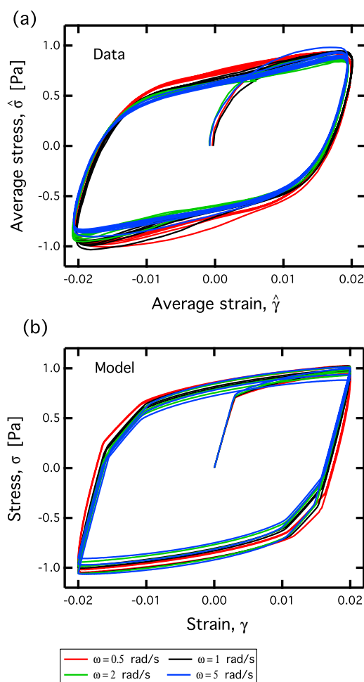
Fig. 16 Frequency dependent behavior under LAOS at moderate strain amplitudes ( \gamma_0 = 2\% ) for both the 10% model crude oil (a) and the IKH model (b). The IKH model model coefficients are the same as in Figs. 14 and 15.
