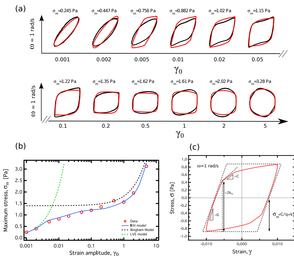
Fig. 14 Modeling of the alternate state in (a) of LAOS tests shown in Fig. 10 ( \omega = 1 rad/s). Model parameters are C/q = 0.7 Pa, \mu_p = 0.42 Pa.s, k_3 = 0.7 Pa, k_1/k_2 = 0.033 s ^{-1} , G = 250 Pa, \eta = 500 Pa.s, k_1 = 0.1 s ^{-1} , C = 70 Pa, m = 0.25 . The red line is the IKH model, the black line shows data for a 10% model crude oil. In (b) the prediction of the maximum stress \sigma_m from the IKH model is compared to the experimentally measured values of \sigma_m . The predictions of a Maxwell LVE model (green dashed line) and a Bingham model (black dotted line) are also shown. Fig. 14 (c) illustrates the key features of the rhomboidal Lissajous curve for the IKH model, when \gamma_0 = 1\% .
