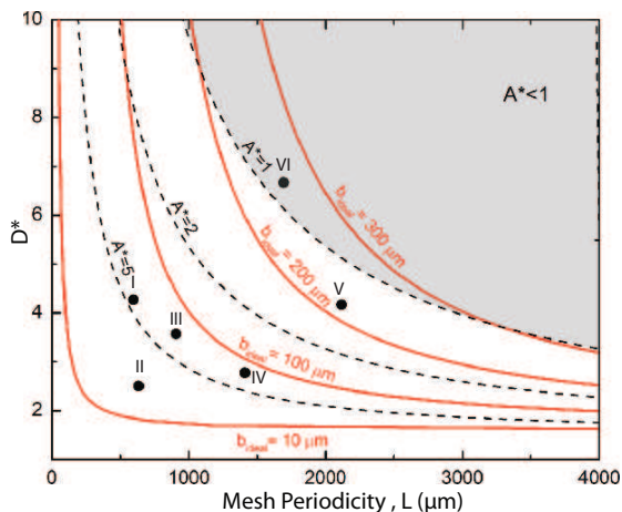
Fig. 7 The design chart for ideal flat non-wetting mesh surfaces, with contours of fixed slip length plotted as solid red lines (from Eq. 6) and contours of fixed robustness factor A^* drawn as dashed black lines as a function of the dimensionless spacing ratio D^* = (R + D)/R and the mesh periodicity L = 2D + 2R . The shaded region indicates parts of the design space where A^* < 1 and the liquid meniscus will penetrate into the mesh. The data points correspond to the location in the design space of the various superhydrophobic coated meshes used in this study.
