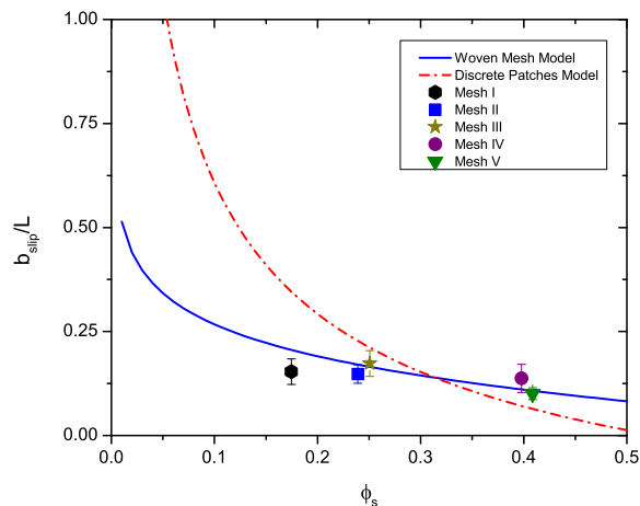
Fig. 10 Ratio of b_{\text{slip}}/L plotted against the solid area fraction r\phi_s for Meshes I-V. The solid blue line and dashed red line correspond to the predictive curves for b_{\text{woven}} (from Eqn. 7) and b_{\text{discrete}} (from Eqn. 3) respectively.
