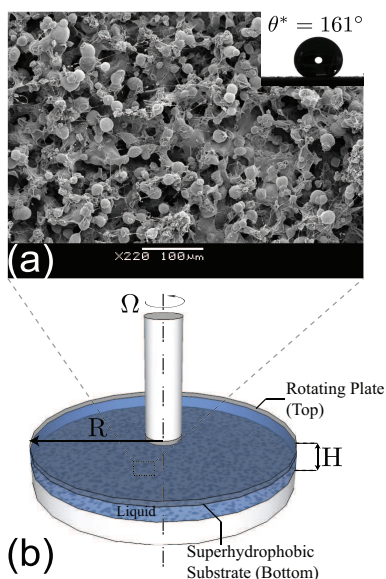
Fig. 2 (a) SEM image of spray-coated superhydrophobic surface displaying corpuscular micro-structured morphology (b) Schematic of plate-plate fixture mounted on a controlled stress rheometer used to quantify apparent slip lengths using a 50 vol% glycerol/water mixture as probe liquid
