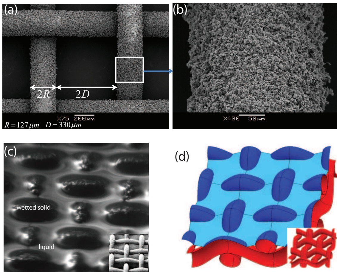
Fig. 6 (a,b) Scanning electron micrographs at different magnifications of the dual-textured spray-coated superhydrophobic mesh surfaces; (c) image of the solid-liquid-vapor composite interface for a 50 vol% glycerol/water solution resting between a spray-coated mesh and the upper rotating plate of the rheometer. The dark regions indicate the wetted area of the mesh and the light regions correspond to reflection of incident light off the liquid meniscus. The inset shows the structure of the spray-coated mesh in the dry state (d) The composite interface on a model sinusoidal woven mesh, simulated using Surface Evolver FEM software. The dark blue, light blue, and red colors represent the wetted solid, liquid-air meniscus and the dry mesh surfaces respectively. The inset depicts the structure of the periodic mesh in the dry state.
