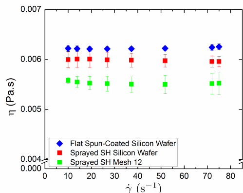
Fig. 3 Apparent viscosities of 50 vol% glycerol/water mixture measured for a gap separation of h = 1000 \mu\text{m} on (i) flat spin-coated hydrophobic surface; (ii) Spray-coated superhydrophobic silicon wafer; (iii) Spray-coated superhydrophobic mesh with wire radius R=254 \mu\text{m} and mesh spacing D=805 \mu\text{m} .
