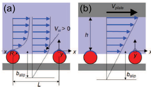
Fig. 1 (a) A schematic diagram showing a liquid flow on a textured non-wetting surface, possessing an effective velocity \bar{V}_w that is averaged over the texture period L . (b) A laminar Couette flow with average shear rate \dot{\gamma}_a = V_{\text{plate}}/h between a non-wetting textured bottom surface exhibiting an average slip length \langle b_{\text{slip}} \rangle and a conventional flat solid top surface possessing a no-slip boundary condition.
