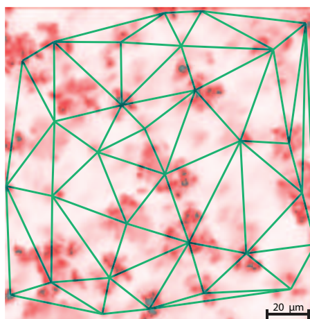
Fig. 5 Confocal Microscope slice image of the spray-coated surface tagged with a Red Nile dye and imaged at the mid-plane. The overlaid lines correspond to the Delaunay triangulation of the centroids of the individual microtextured features (determined from the ImageJ software), and is used to determine the mean periodicity \bar{L}
