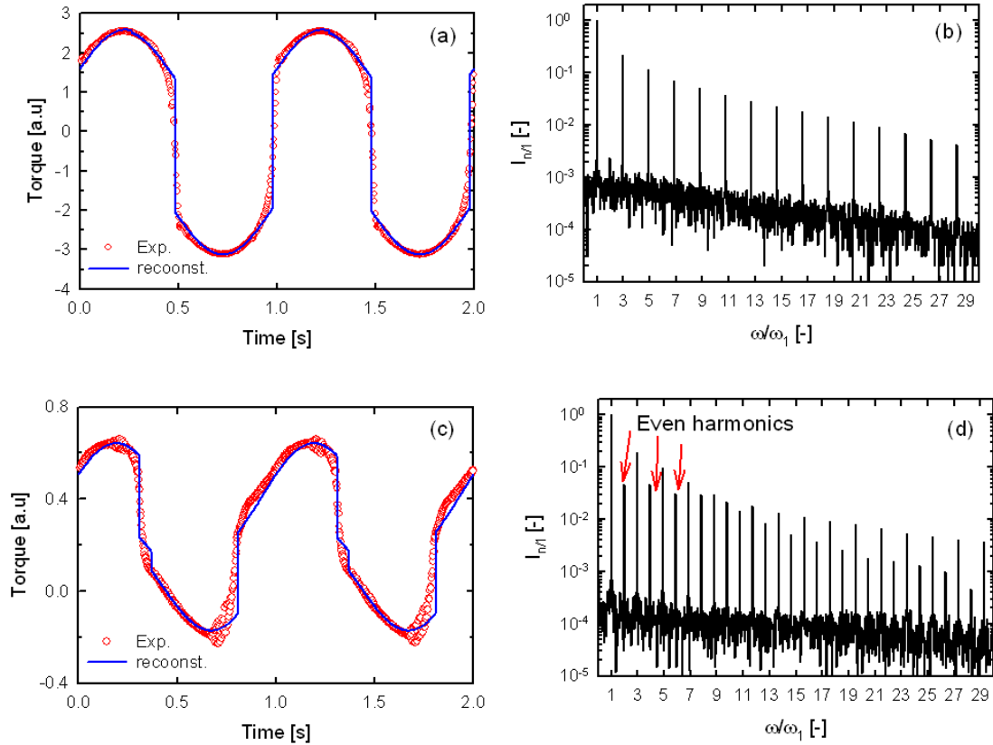
Fig. 29. The overlay of the time-dependent torque response and the reconstructed time data and the corresponding FT spectra of the experimental data for sample 1 ((a) and (b)) and sample 2 ((c) and (d)). The
