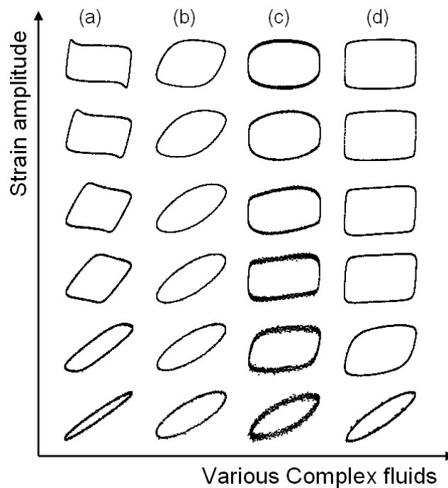
Fig. 11. The Lissajous curves (stress (y axis) vs. strain (x axis))(●) of various complex fluids, arranged from small strain amplitude to large strain amplitude at a fixed frequency, 1rad/s (a) Xanthan gum 4% aqueous solution (b) Hyaluronic acid 1% aqueous solution (c) soft gel of PEO-PPO-PEO triblock 20% aqueous solution (d) hard gel of PEO-PPO-PEO triblock 20% aqueous solution.
