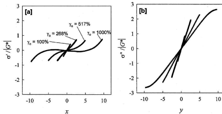
Fig. 23. Decomposition of shear stress into elastic and viscous part for polypropylene melt at 170 °C and 1rad/s. The shear stress is normalized by the complex modulus in the linear regime. (a) elastic stress versus strain x \equiv \gamma = \gamma_0 \sin \omega t (b) viscous stress versus y \equiv \dot{\gamma} / \omega = \gamma_0 \cos \omega t . Reproduced by permission of Cho et al. [65], copyright (2005) of the Society of Rheology.
