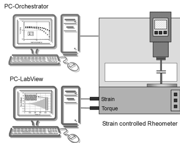
Fig. 3. Experimental set up for common LAOS experiments. The strain, torque and normal forces are digitized via a stand-alone PC. The rheometer is controlled via a second PC with the standard instrument software.
