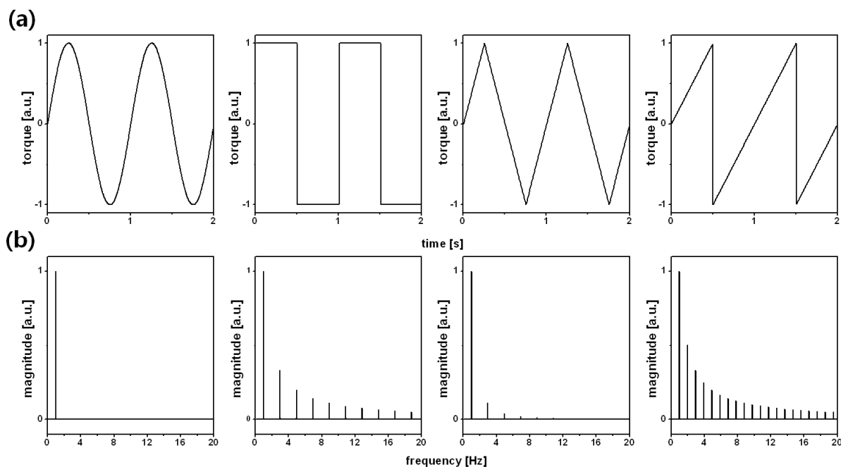
Fig. 22. The four characteristic functions (from left to right): a sine, a rectangular, a triangular and a saw tooth shaped wave, representing viscoelastic, strain softening, strain hardening, and shear bands. The time domain data is displayed on the top (a) and the corresponding FT magnitude spectra in the bottom (b). Reproduced by permission of Klein et al. [5], copyright (2007) of American Chemical Society.
