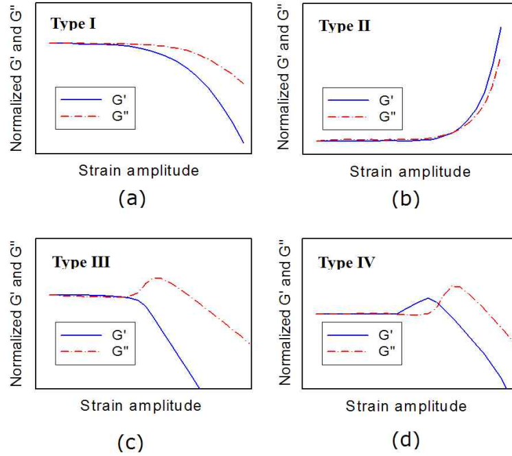
Fig. 5. The four archetypes of LAOS behavior as outlined by Hyun et al. [62]; (a) strain thinning (b) strain hardening (c) weak strain overshoot (d) strong strain overshoot. Reproduced by permission of Hyun et al. [62], copyright (2002) of Elsevier.
