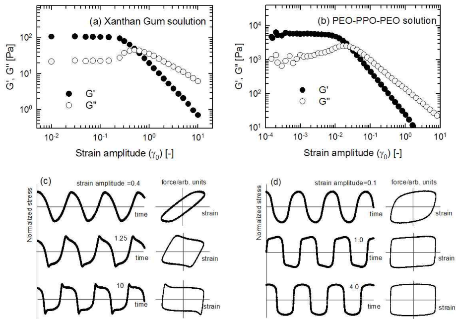
Fig. 7. The viscoelastic moduli G'(\gamma_0) and G''(\gamma_0) for (a) Xanthan gum 4 wt% aqueous solution at \omega = 1\text{ rad/s} and T = 25\text{ }^\circ\text{C} and (b) hard gel of PEO-PPO-PEO triblock 20 wt% aqueous solution at \omega = 1\text{ rad/s} and T = 26\text{ }^\circ\text{C} are shown. Both aqueous solutions display LAOS type III (weak strain overshoot) behavior. However, the shapes of the nonlinear stress waveforms are markedly different. The stress data and Lissajous patterns are shown in (c) xanthan gum 4% aqueous solution (saw tooth shape) and (d) hard gel of PEO-PPO-PEO triblock 20% aqueous solution (rectangular shape). The different shape of these stress waveforms originates from different microstructures. Reproduced by permission of Hyun et al. [94], copyright (2003) of the Korean Society of Rheology and the Australian Society of Rheology.
