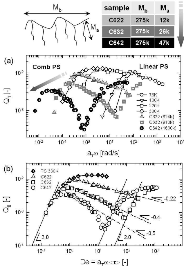
Fig. 27. (a) Frequency dependence of the zero-strain nonlinearity Q_0 for linear PS chains (PS 76K, 100K, 220K, 330K) and PS combs (C622, C632 and C642) at T_{\text{ref}} = 190 °C. With increasing molecular weight of the branched chain ( M_a ), the maximum corresponding backbone chain ( Q_{0,b} ) is decreasing. (b) For clear comparison, the coefficient Q_0 is plotted against Deborah number ( De = a_T \omega \langle \tau \rangle ) of linear PS 330K and comb PS (C622, C632 and C642) at T_{\text{ref}} = 190 °C. Reproduced by permission of Hyun et al. [42], copyright (2009) of American Chemical Society.
