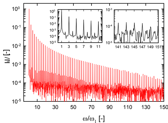
Fig. 19. FT-Rheology spectra at \omega_1/2\pi = 0.1 \text{ Hz} of an emulsion. Mechanical overtones up to the 151-st order could be detected.
