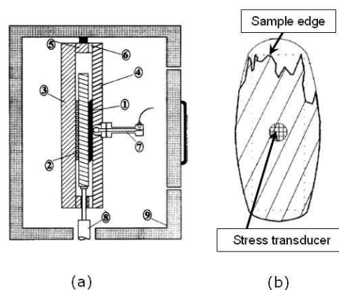
Fig. 2. (a) Cross-section showing the essential elements of a sliding plate rheometer incorporating an elastic type shear stress transducer: ① sample ② moving plate ⑦ shear stress transducer. (b) The schematic sample shape under LAOS is shown with flow heterogeneity at the sample edge, because the stress transducer is
