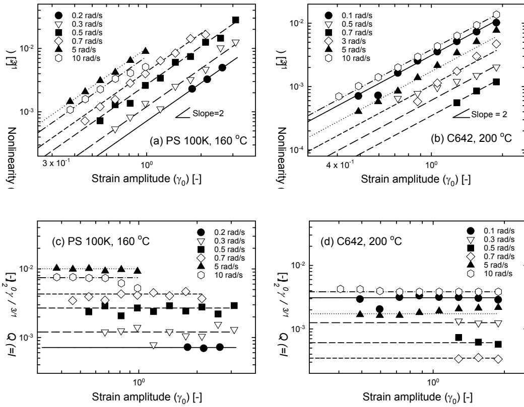
Fig. 26. The nonlinear intensity ratio ( I_{3/1} ) as a function of strain amplitude for linear and comb PS at various frequencies; (a) linear monodisperse polystyrene (PS 100K) at 160 °C (b) entangled branched melt C642 at 200 °C. Also shown are the corresponding values of the Q coefficient as a function of strain amplitude evaluated from the intensity ratio data for (c) PS 100K at 160 °C and (d) C642 at 200 °C. Reproduced by permission of Hyun et al. [42], copyright (2009) of American Chemical Society.
