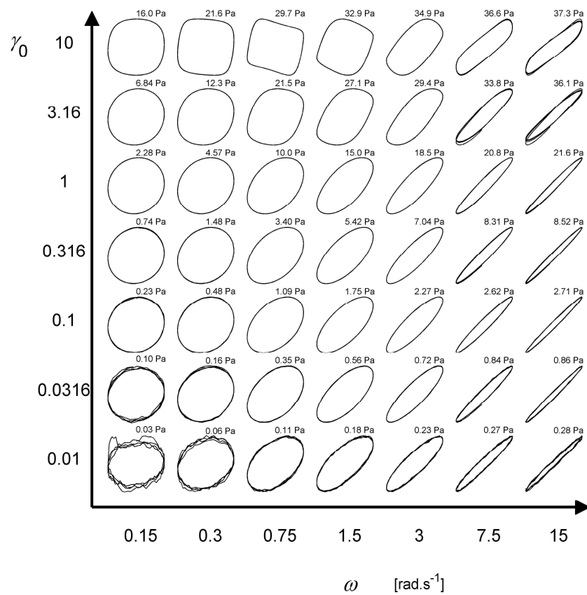
Fig. 12. Raw LAOS data for a micellar solution, generated from experimental oscillatory tests, shown as normalized elastic Lissajous curves of stress \sigma(t) vs. strain \gamma(t) . Each trajectory is positioned in a Pipkin space according to the imposed values of strain amplitude \gamma_0 and frequency \omega . Solid lines are total stress \sigma(t)/\sigma_{\max} vs. \gamma(t)/\gamma_0 . The maximum stress \sigma_{\max} is indicated above each curve. Reproduced by permission of Ewoldt et al. [68], copyright (2009) of The Society of Rheology.
