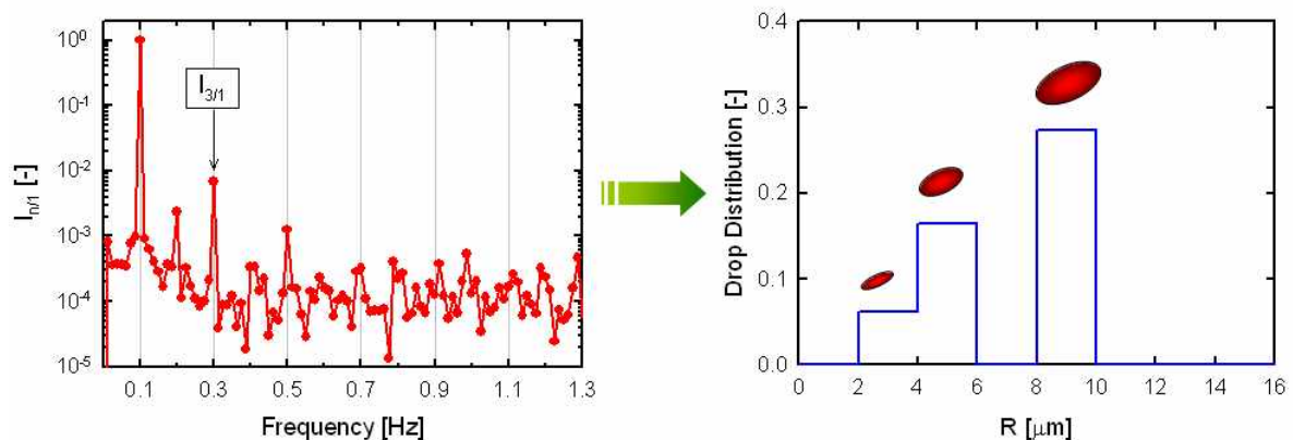
Fig. 31. Drop distribution estimated with the regression procedure for blend C (10% PDMS and 90% PIB) using the FT-rheology spectra. Reproduced by permission of Carotenuto et al. [45], copyright (2009) of American Chemical Society.
