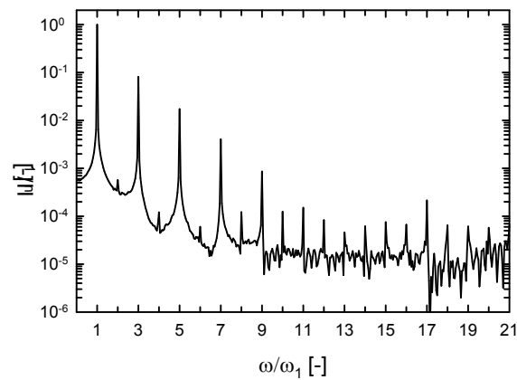
Fig. 17. FT-Rheology spectra of polyvinylalcohol (PVA) solution, at T = 5\text{ }^\circ\text{C} , \gamma_0 = 20 , frequency 1Hz, where a S/N ratio of 100,000 : 1 could be achieved. Reproduced by permission of Wilhelm [32], copyright (2003) of WILEY-VCH.
