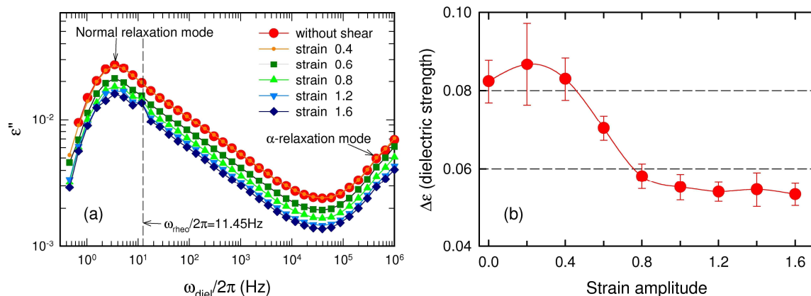
Fig. 38. (a) The dielectric loss \varepsilon'' as a function of dielectric frequency under LAOS with PI 55K at 10^\circ\text{C} . The LAOS tests were carried out at a rheological test frequency \omega_{\text{rheo}}/2\pi = 11.45\text{Hz} . (b) The dielectric strength as a function of strain amplitude is divided into three regions for the PI 55K, an initially constant value ( 0 < \gamma_0 < 0.4 ), decreasing ( 0.4 < \gamma_0 < 1 ), and asymptotic plateau at high strains ( \gamma_0 > 1 ). Reproduced by permission of Hyun et al. [174], copyright (2009) of Elsevier.
