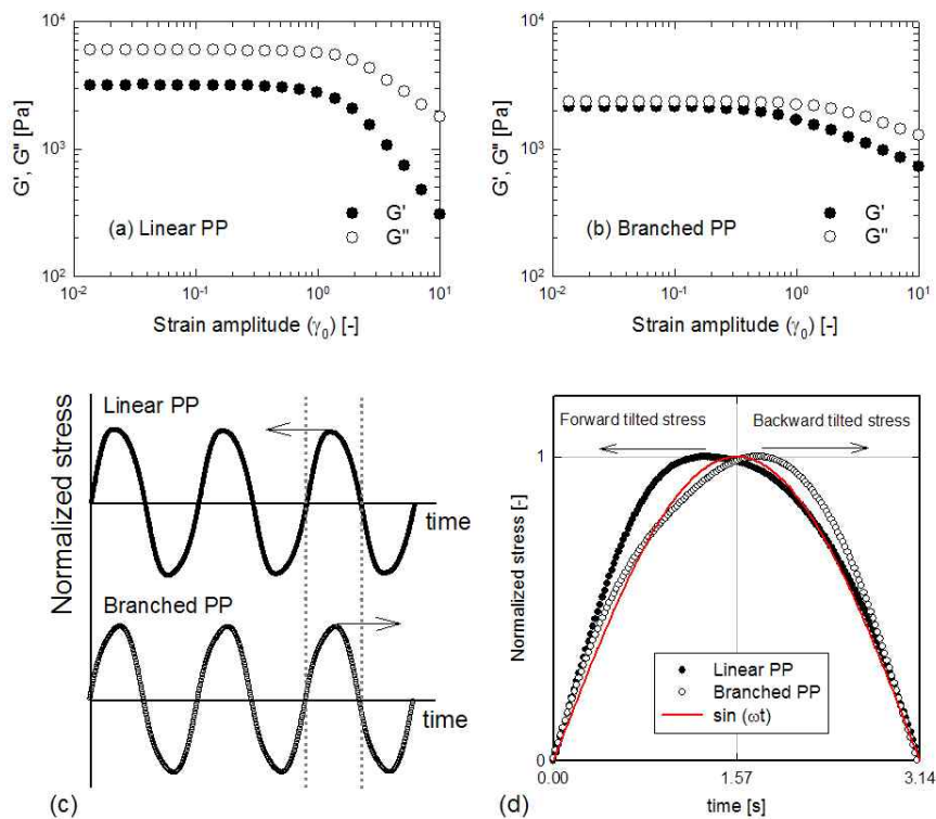
Fig. 6. The viscoelastic moduli G'(\gamma_0) and G''(\gamma_0) at \omega = 1 \text{ rad/s} and T = 180 \text{ }^\circ\text{C} for two different Polypropylene
