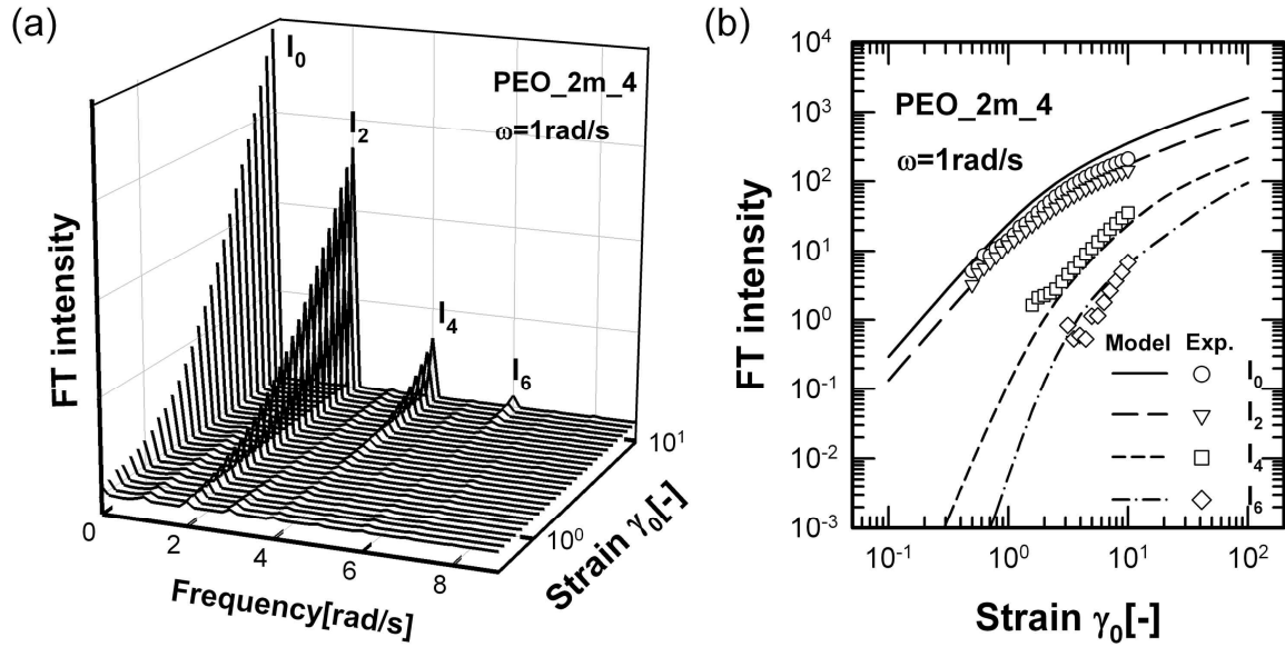
Fig. 21. (a) 3D plot for the FT of the oscillating first normal stress difference for a 4wt% PEO solution with a molecular weight 2 \times 10^6 g/mol. There are trace contributions from the odd harmonics for the entire range of strain amplitudes tested. (This non-idealized behavior is similar to the even harmonics present in the nonlinear shear stress.) (b) FT intensity as a function of strain amplitude. The experimental data are compared with simulations using a multi-mode Giesekus model [123]. Experimental measurements of the higher harmonic intensities ( I_4 , I_6 ) have severe errors at low strain amplitude.
