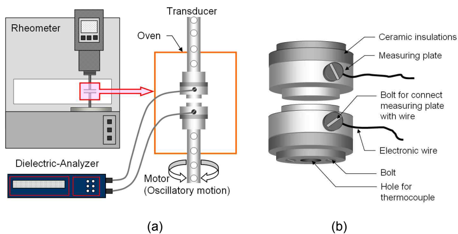
Fig. 37. (a) Experimental setup for the in situ combination of rheometry and dielectric spectroscopy. (b) Schematic 3-D view of the measurement geometry, which consists of parallel electrode plate, ceramic insulation, and bolts for connecting the measuring plate with the electronics. Reproduced by permission of Hyun et al. [174], copyright (2009) of Elsevier.
