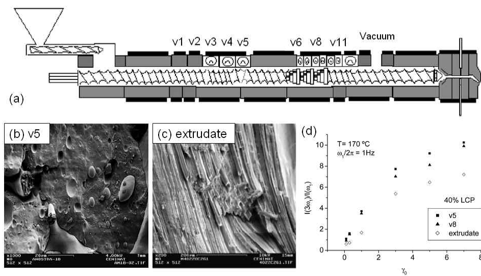
Fig. 32. (a) Screw and cylinder profile used for the processing of the blends. Here “vi” is i-th valve that allows local removal of samples along the extruder length. Morphological evolution along the length for the blend with 40 wt% LCP processed at 220^\circ\text{C} (SEM) (b) location v5 in the extruder and (c) final extrudate. (d) ratio I_{3/1} from FT-rheology as a function of the applied strain amplitude for the different samples collected along the extruder length (blend with 40wt % LCP at 170^\circ\text{C} ). Reproduced by permission of Filipe et al. [46], copyright (2004) of Elsevier Science.
