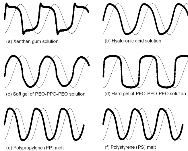
Fig. 10. Stress curves (●) and applied strain curves (—) as a function of time for various complex fluids at large strain amplitude and frequency 1rad/s. (a) Xanthan gum 4 wt% aqueous solution at strain amplitude \gamma_0 = 10 (b) Hyaluronic acid 1% aqueous solution at strain amplitude \gamma_0 = 7.2 (c) soft gel of PEO-PPO-PEO triblock 20 wt% aqueous solution at strain amplitude \gamma_0 = 10 (d) hard gel of PEO-PPO-PEO triblock 20% aqueous solution at strain amplitude \gamma_0 = 4 (e) Polypropylene (PP) melt at strain amplitude \gamma_0 = 10 (f) Polystyrene (PS) melt at strain amplitude \gamma_0 = 10 .
