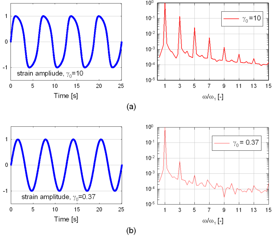
Fig. 18. The stress curve and FT spectrum of Hyaluronic acid 1% aqueous solution at frequency, \omega_1 = 1 \text{ rad/s} . (a) Normalized stress and FT spectrum at strain amplitude \gamma_0 = 10 . A non-sinusoidal shape is observed, and the FT-method quantifies the extent of the nonlinear response via the magnitude (and phase) of the odd higher harmonics. (b) Normalized stress and FT spectrum at a strain amplitude \gamma_0 = 0.37 , which corresponds to intermediate strain amplitude. To a naked eye, the time-dependent stress is similar to a perfect sinusoid. However, the presence of a 3 rd harmonic is clearly shown by the Fourier spectra.
