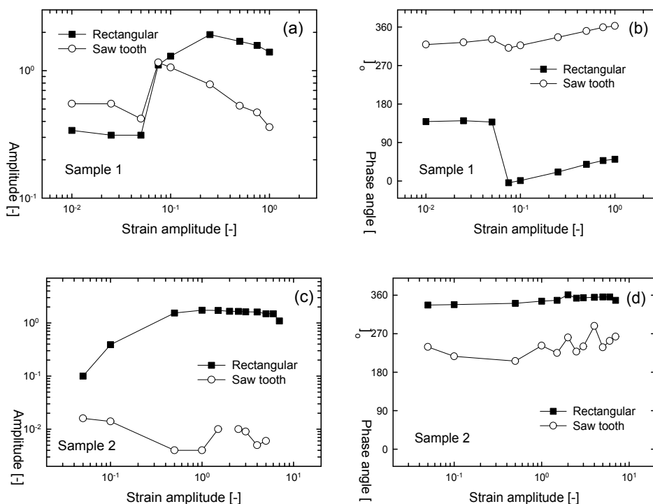
Fig. 30. Dependence of the amplitude and the phase angle on the strain amplitude of the characteristic functions for sample 1 ((a) amplitude and (b) phase angle) and sample 2 ((c) amplitude and (d) phase angle). The characteristic response contains strain softening (rectangular basis function) and wall slip or shear banding (saw tooth wave form). In rare cases, experimental problems such as wall slip appeared. In those cases the data is not shown. Reproduced by permission of Klein et al. [5], copyright (2009) of American Chemical Society.
