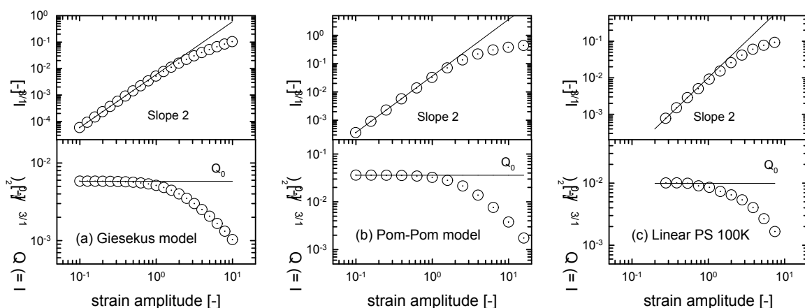
Fig. 20. I_{3/1} and Q function of strain amplitude from medium strain amplitude ( \gamma_0 \approx 0.1 ) to large strain amplitude ( \gamma_0 \approx 10 ) (a) Giesekus model with G=1 , \lambda=1 , \alpha=0.3 , \omega/2\pi = 1 Hz, (b) integral pom-pom model with q=5 , s_a=6 and s_b=20 , \omega/2\pi = 0.1 Hz, and (c) monodisperse linear PS (PS 100K) at \omega = 4.25 rad/s, T = 160 °C.
