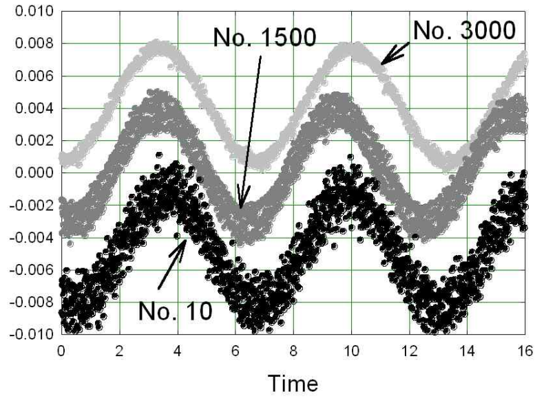
Fig. 4. The torque as a function of time for Xanthan gum 4% aqueous solution at fixed strain amplitude, \gamma_0 = 0.03 with strain controlled rheometer RMS 800 that can detect a torque within the range 2-2000 mN·m. The torque is shifted vertically for ease of comparison. Increasing the oversampling number reduces the noise while the absolute torque amplitude remains the same.
