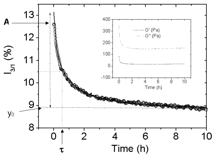
Fig. 33. Variation of the relative intensity of the third harmonic I_{3/1} (O) during the 10 hours of the macroscopic orientation process of a styrene-butadiene (9 kg/mol-9kg/mol) sample. The solid line represents the stretched exponential fit. The insert represents the variation of the storage modulus and the loss modulus as a function of time. Reproduced by permission of Oelschlaeger et al. [49], copyright (2007) of WILEY-VCH.
