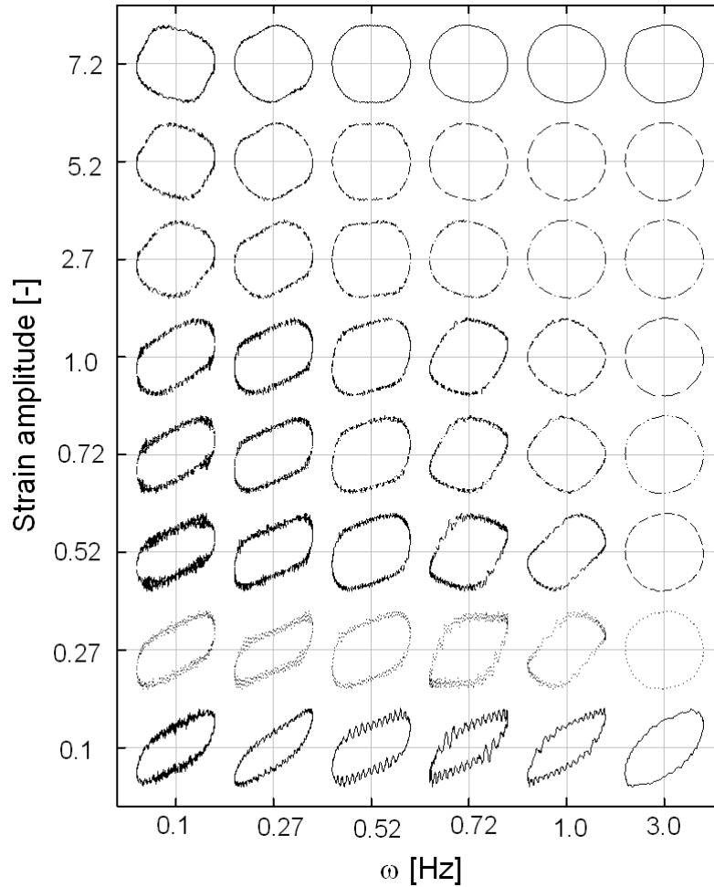
Fig. 13. Raw LAOS data for a highly concentrated suspension system (50wt% PMMA particle (100 nm Radius) in paraffin oil), generated from experimental oscillatory tests, shown as normalized elastic Lissajous curves of stress \sigma(t) vs. strain \gamma(t) . Each trajectory is positioned in a Pipkin space according to the imposed values of strain amplitude \gamma_0 and frequency \omega .
