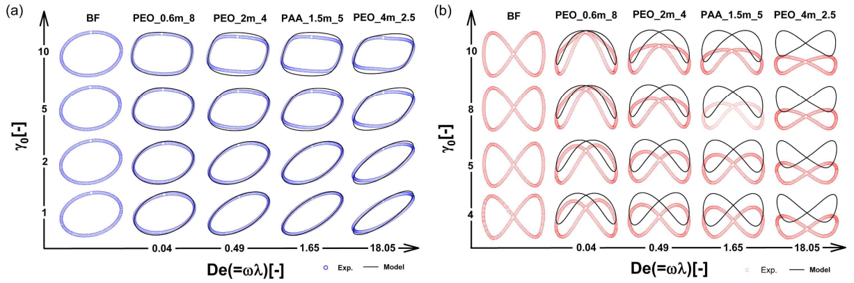
Fig. 16. The experimental Lissajous patterns obtained for various polymer solutions; BF (Boger fluid), PEO (Poly ethylene oxide) and PAA (Poly acryl amide) solutions at a range of concentrations (a) The loop for shear stress vs. strain, (b) the loop for first normal stress difference vs. strain. The results are arranged in a Pipkin space (strain amplitude vs. frequency ( De = \omega/\omega_c , \omega_c is crossover frequency at G' = G'' )). For four aqueous polymer solutions, the experimental data (symbols) are compared with model data (lines). For the Boger fluid only the experimental data is shown.
