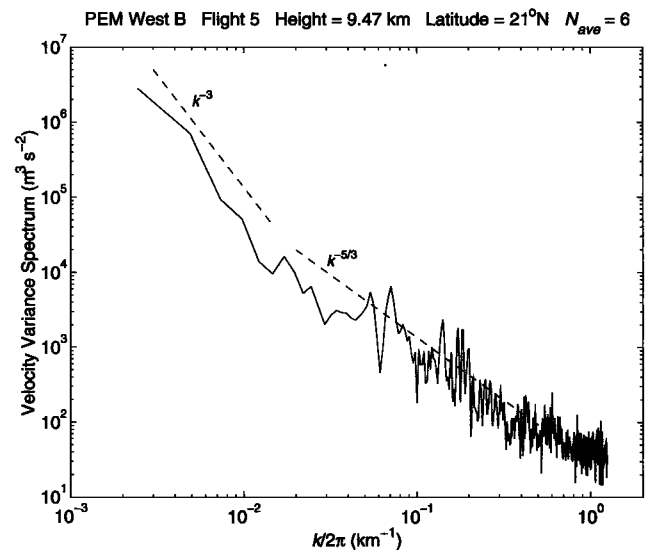
Figure 15. Horizontal velocity variance spectra (the sum of zonal and meridional velocity variance spectra) for one straight-and-level flight segment during PEM-West B flight 5 from February 8, 1994, 2037 UT to February 9, 1994, 0002 UT. The start and end coordinates were 21^\circ 10'N , 160^\circ 20'W and 20^\circ 30'N , 176^\circ 10'W . FFTs were taken over six consecutive 2048-s segments. As guides to the eye, dashed lines indicating log-log slopes of -3 and -5/3 are also included.
