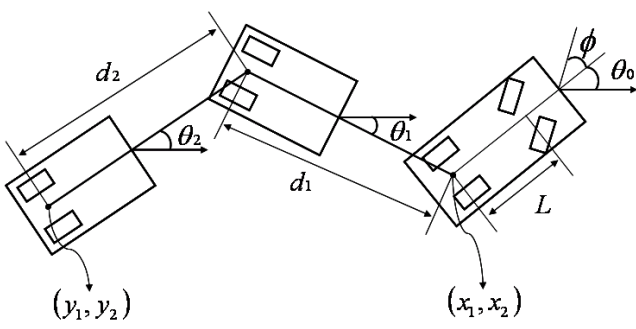
Fig. 1. Parameters for a car pulling k -trailers
